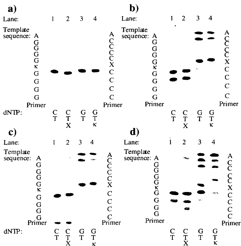
Fig. 2 PAGE analysis of primer extension reaction by (a) Vent, (b) Deep Vent, (c) HotTub, and (d) 9^{\circ}\text{N} DNA polymerase. Deoxynucleoside triphosphates present in solution are indicated below (50 \mu\text{M} each). Incubations were performed at 75^{\circ}\text{C} for 15 min with 0.15 pmol labeled primer/template-complex containing either the d(pyDAD) nucleobase (lanes 1-2) or dX (lanes 3-4) and 0.2 units enzyme in a final volume of 25 \mu\text{l} . X stands for 2'-deoxyxanthosine and \kappa for the d(pyDAD) nucleobase, respectively.
